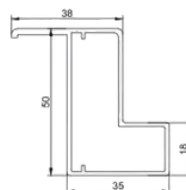
Z Frame Flat
