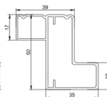
Z Frame Beaded
